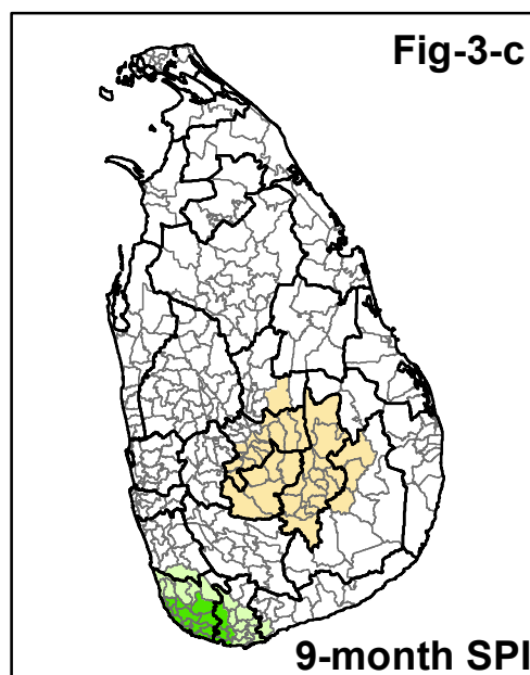
Fig 3 : 3 month (3-a), 6 month (3-b), 9 month (3-c) , 12 month (3-d) , and 18 month (3-e) SPI values through the end of July 2023 for the 331 Divisional Secretariat Divisions (DSD) in Sri Lanka
