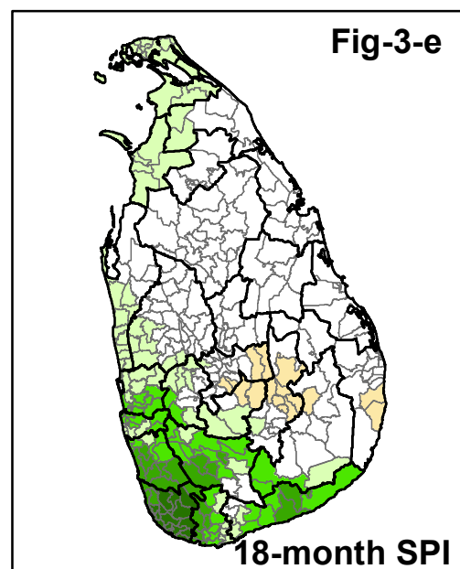
Fig 3 : 3 month (3-a), 6 month (3-b), 9 month (3-c) , 12 month (3-d) , and 18 month (3-e) SPI values through the end of September 2023 for the 331 Divisional Secretariat Divisions (DSD) in Sri Lanka
