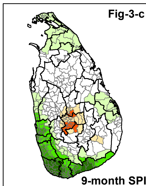
Fig 3 : 3 month (3-a), 6 month (3-b), 9 month (3-c) , 12 month (3-d) , and 18 month (3-e) SPI values through the end of September 2023 for the 331 Divisional Secretariat Divisions (DSD) in Sri Lanka
