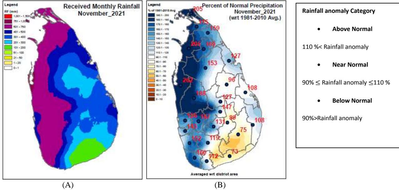
Fig 4: Observed rainfall during month of November 2021
