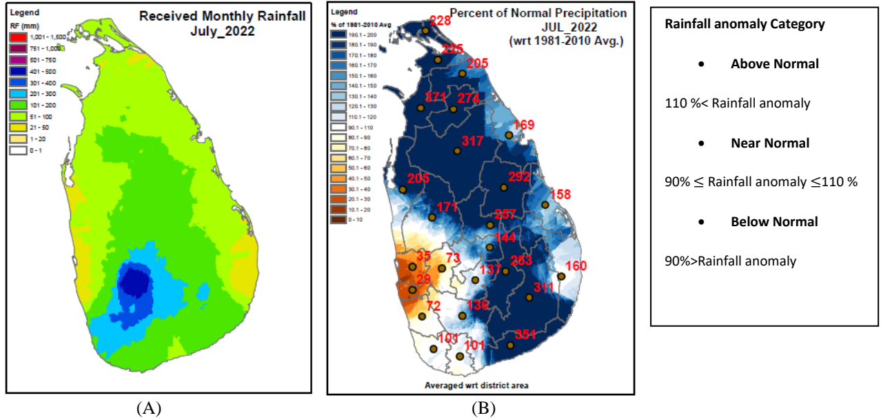
Fig 4: Observed rainfall during month of July 2022
