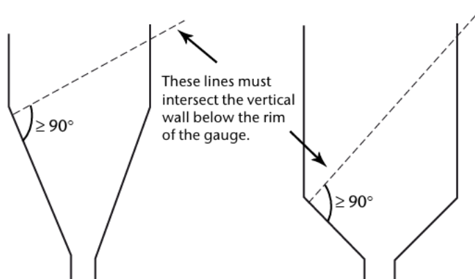
Suitable collectors for raingauges
