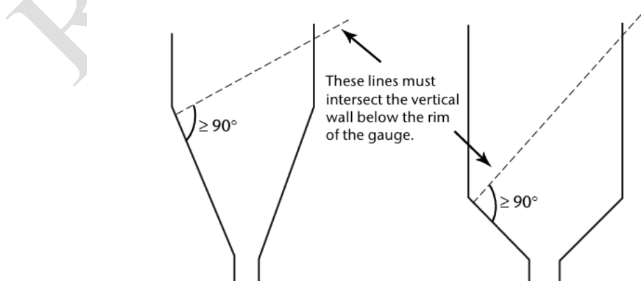
Suitable collectors for raingauges
