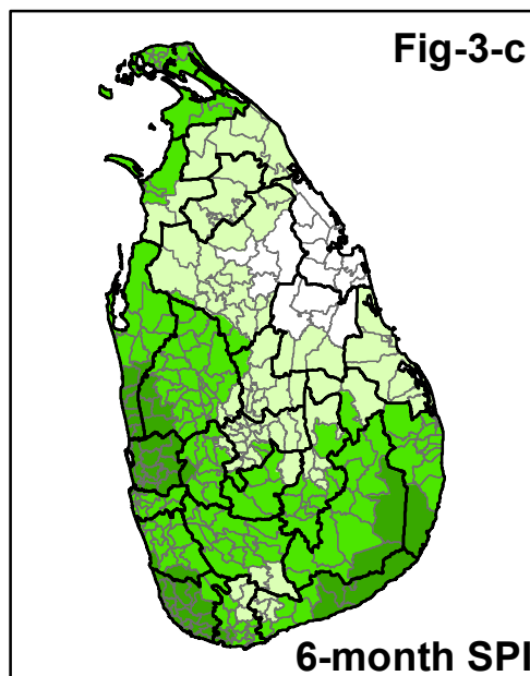
Fig 3 : 1 month (3-a), 3 month (3-b), 6 month (3-c) , 9 month (3-d) , and 12 month (3-e) SPI values through the end of April 2024 for the 331 Divisional Secretariat Divisions (DSD) in Sri Lanka
