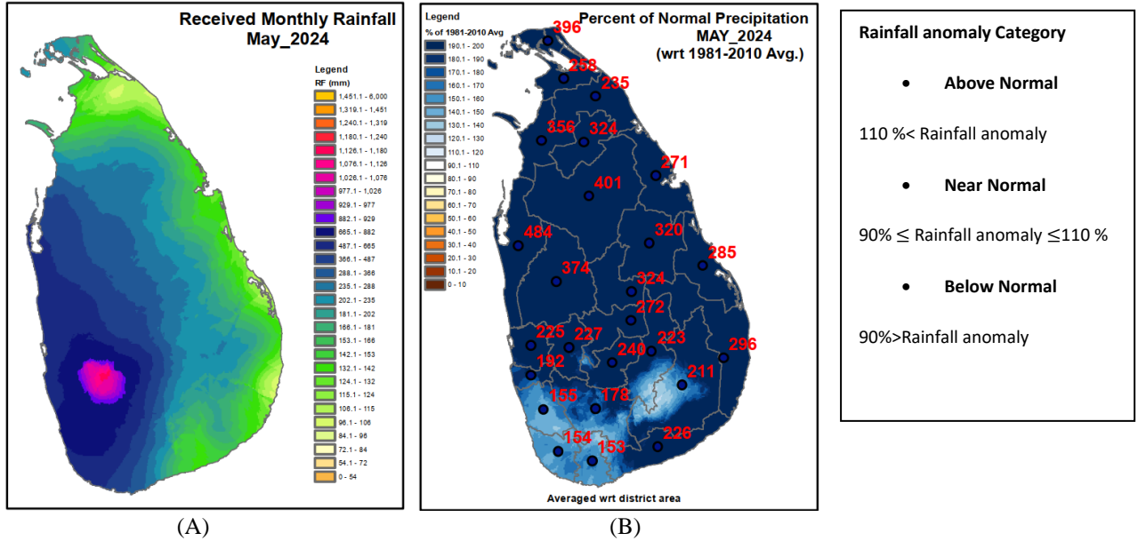
Fig 1: Observed rainfall during the month of May 2024
