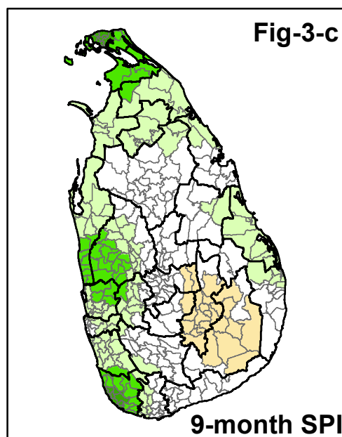
Fig 3 : 3 month (3-a), 6 month (3-b), 9 month (3-c) , 12 month (3-d) , and 18 month (3-e) SPI values through the end of June 2021 for the 331 Divisional Secretariat Divisions (DSD) in Sri Lanka
