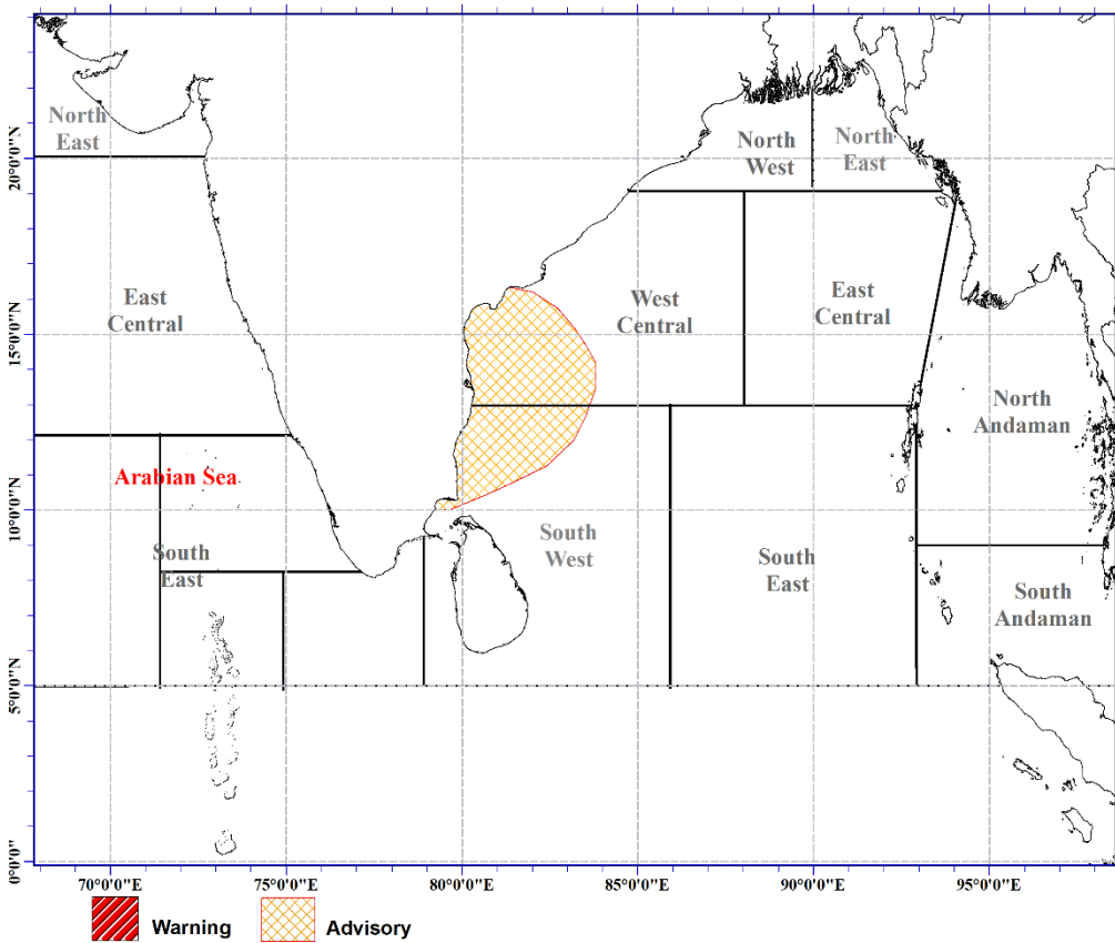
Advisory for low pressure area over Southwest Bay of Bengal. Issued at 03.00 p.m. on 16 May 2026 for the period until 03.00 p.m. 17 May 2026.
